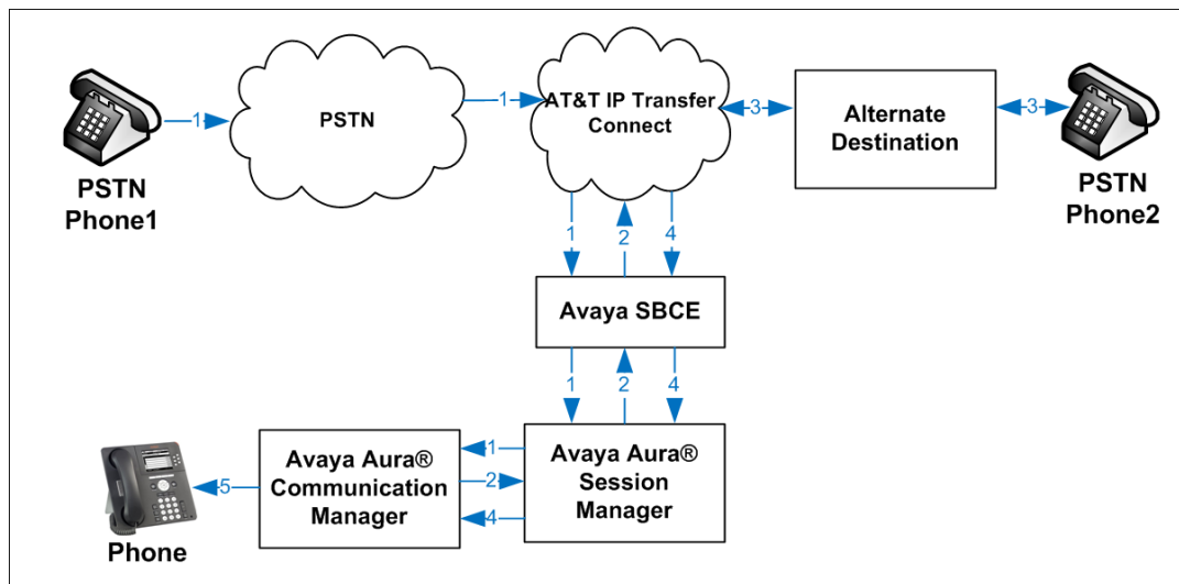
Figure 5: Inbound IPTC Call - Unsuccessful SIP REFER Redirection/Reroute.
