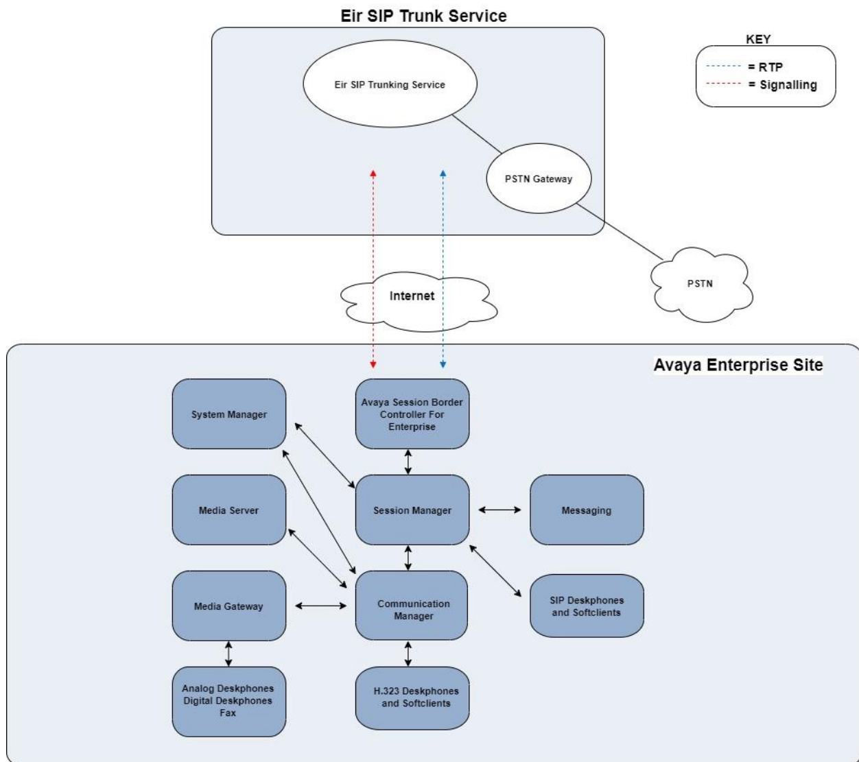
Figure 1: Test Setup Eir SIP Service to Avaya Enterprise
