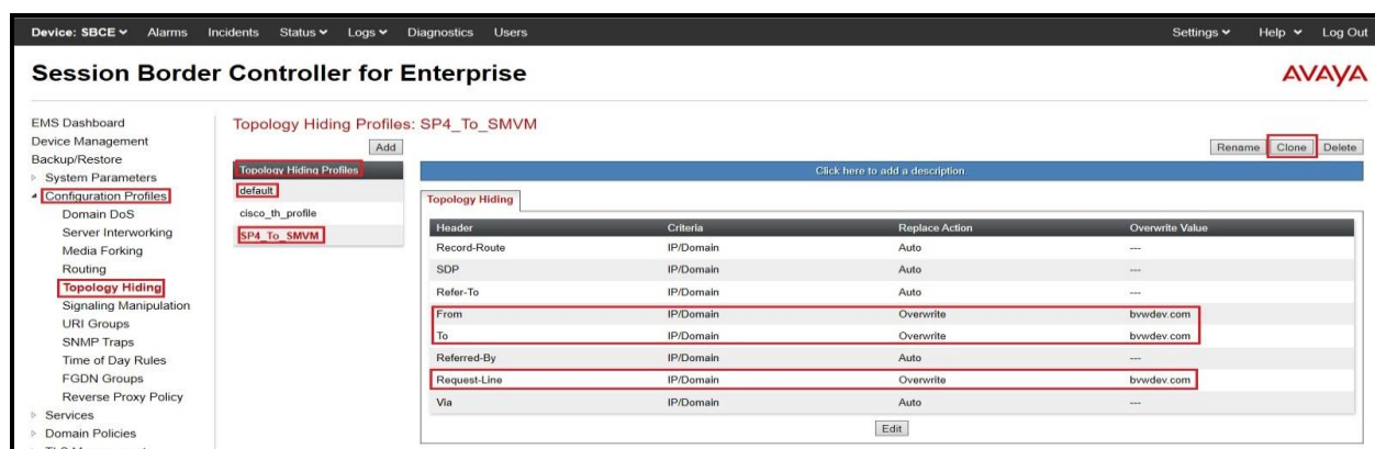
Figure 70: Topology Hiding To Session Manager
