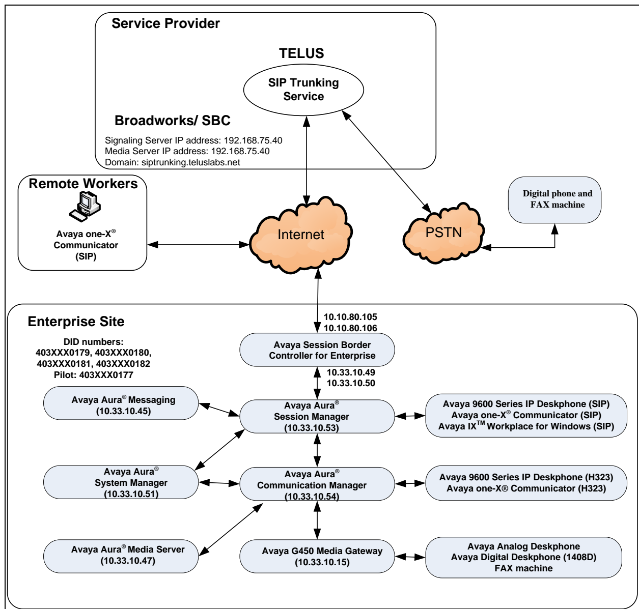
Figure 1: Avaya IP Telephony Network and TELUS SIP Trunk
