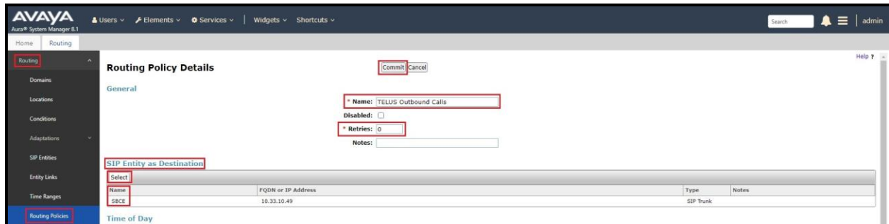
Figure 50: Routing to TELUS SIP Trunk
