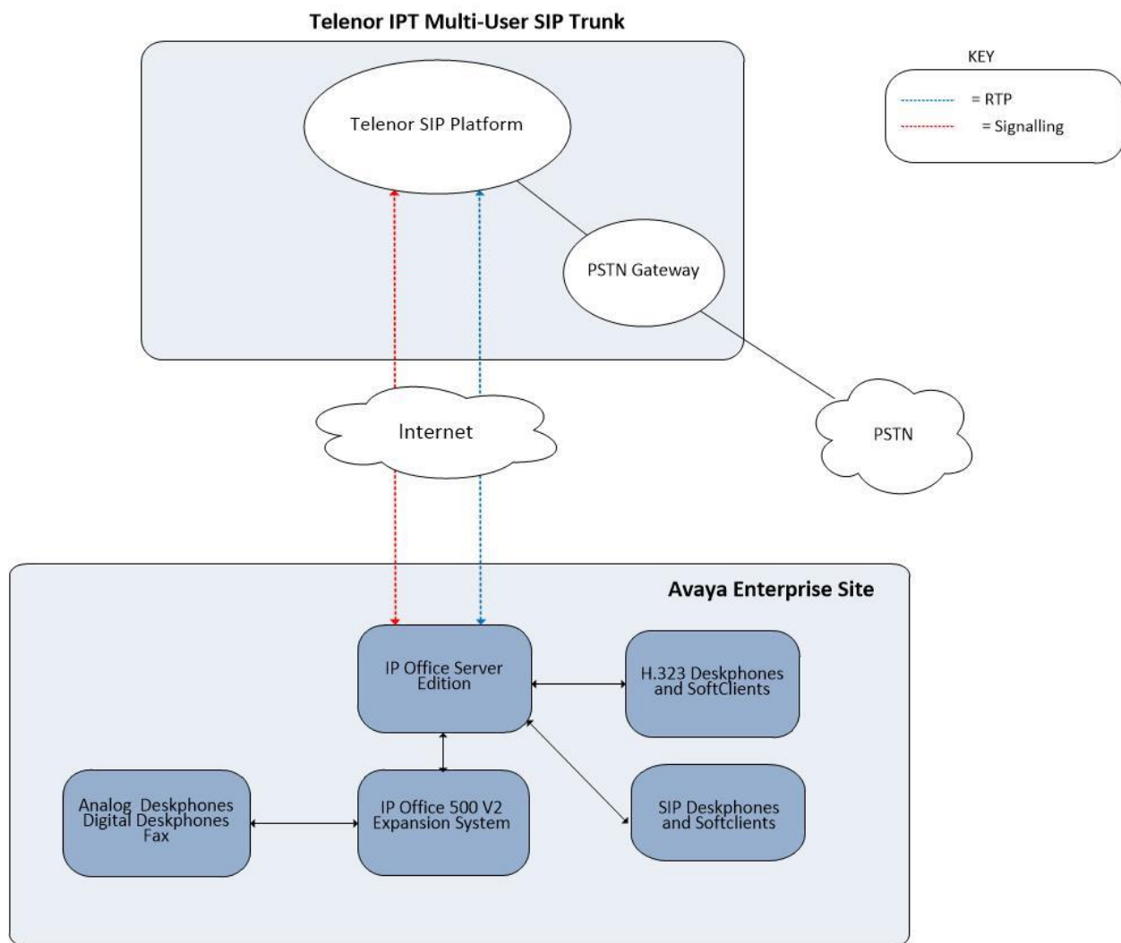
Figure 1: Test Setup Telenor IPT Multi-User SIP Trunk to Avaya Enterprise
