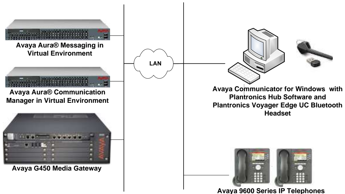
Figure 1: Avaya Communicator for Windows with Plantronics Hub Software and Plantronics Voyager Edge UC Bluetooth Headset
